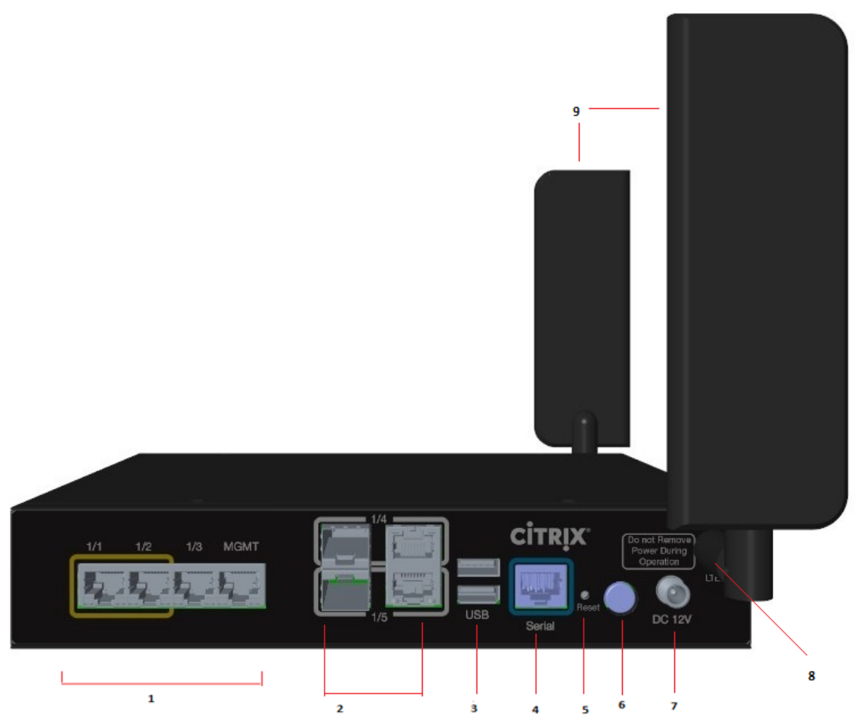
Figure 4. 210 SE (LTE) back panel with antenna
