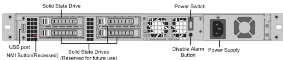
Figure 2. Citrix SD-WAN 2000 PE appliance, back panel
